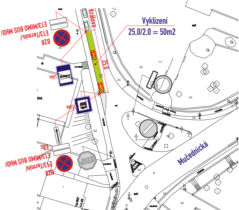
DETAIL 3:
