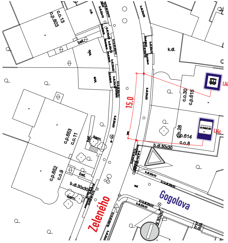
DETAIL 4:
