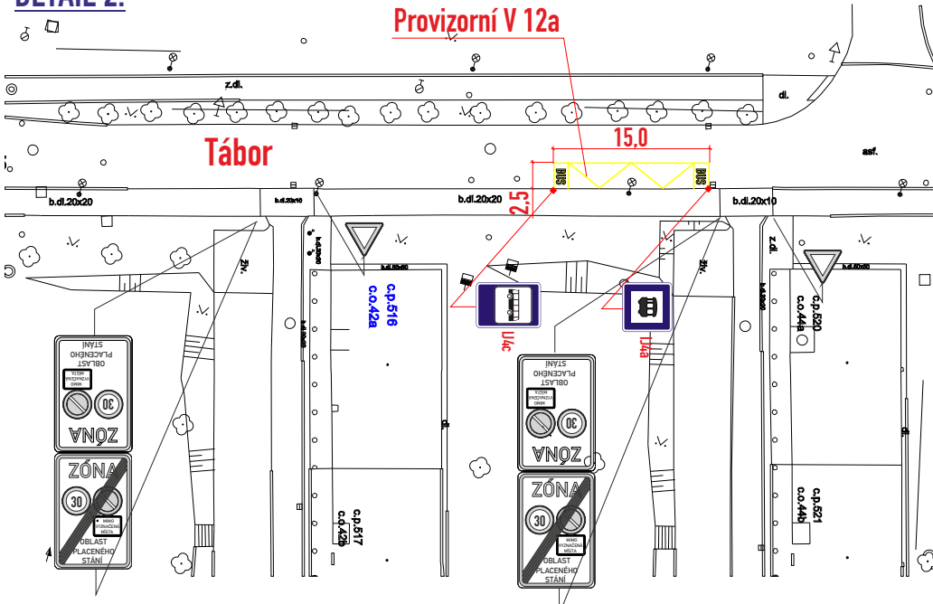
DETAIL 2:
