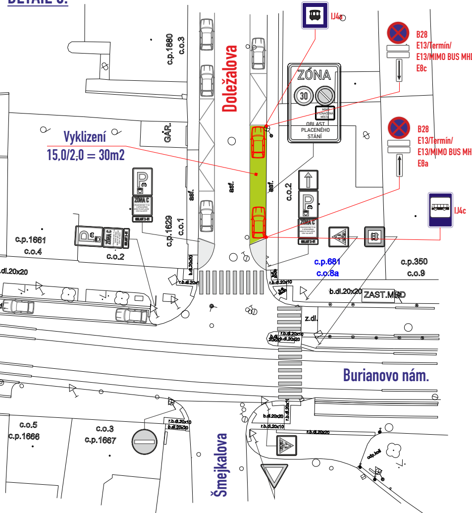
DETAIL 5:
